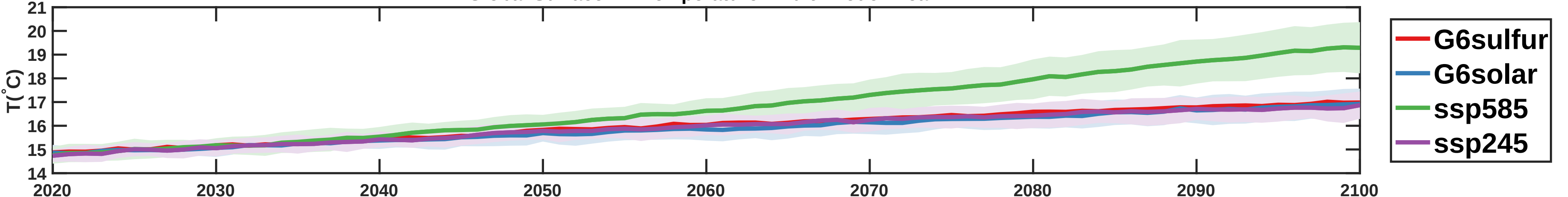
Global Surface Air Temperature - Multi-model mean
