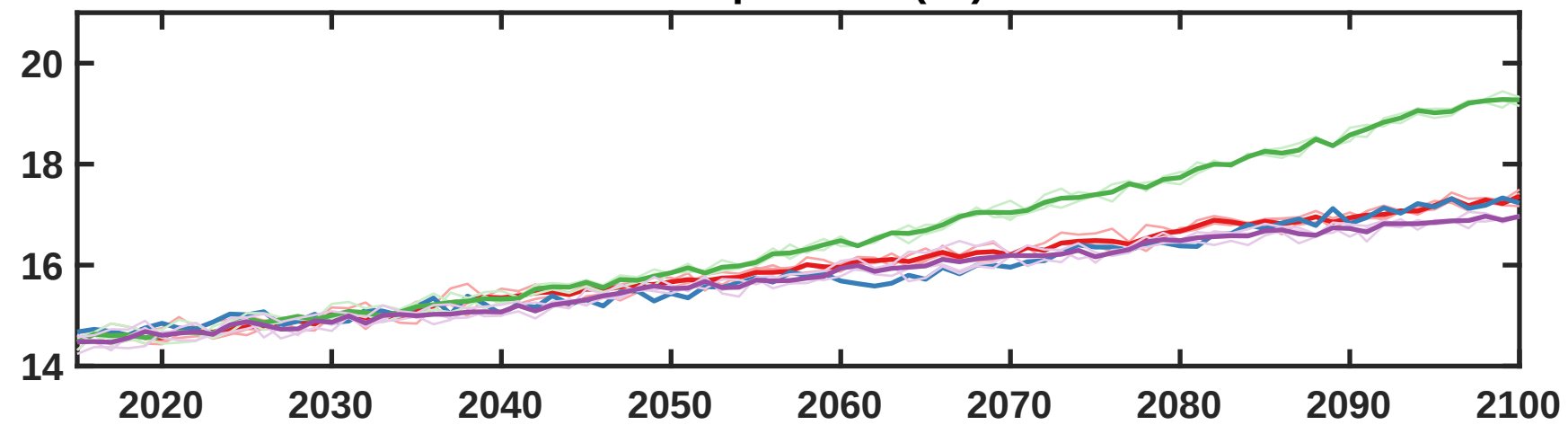
Global Surface Air Temperature (°C) - CNRM-ESM2-1
