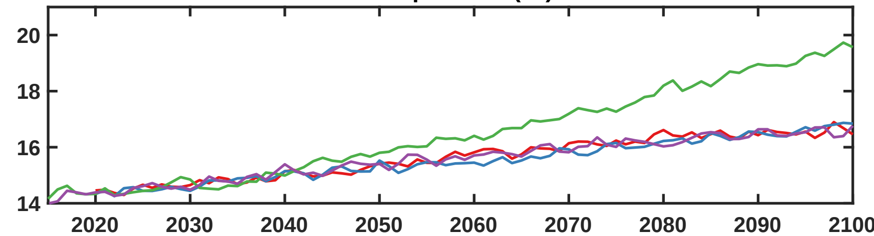
Global Surface Air Temperature (°C) - IPSL-CM6A-LR
