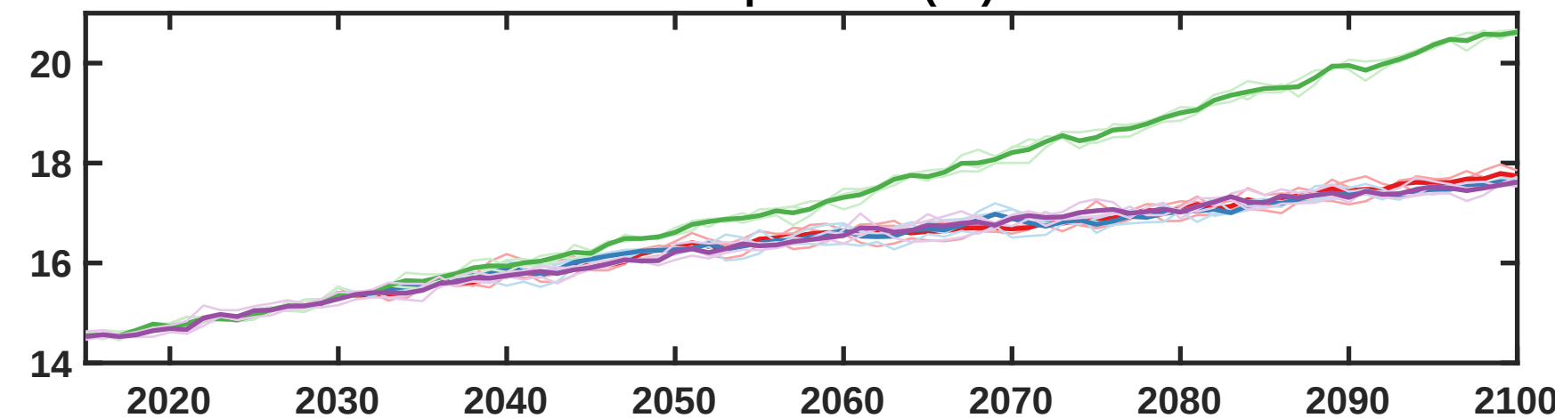
Global Surface Air Temperature (°C) - UKESM1-0-LL
