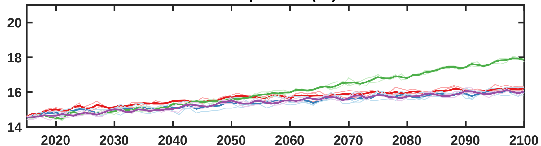
Global Surface Air Temperature - Multi-model mean
