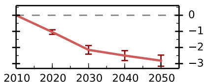
Methane
