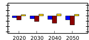
All
