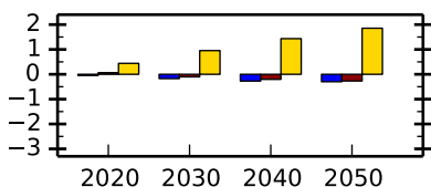
All
