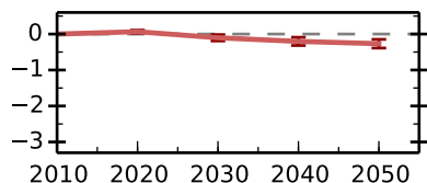
Methane
