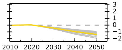
All
