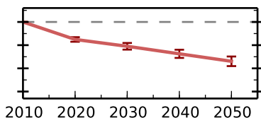
Methane
